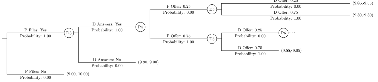
Figure 5: Stage II: filing, answer/default, and a single round of simultaneous offers.
